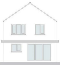
WEST ELEVATION AS PROPOSED 1:100
